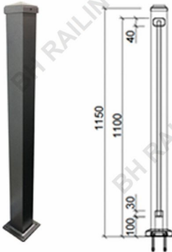
Universal Aluminum Post With Welded Base Plate
