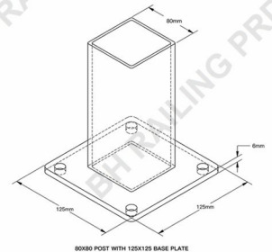
Post Size
