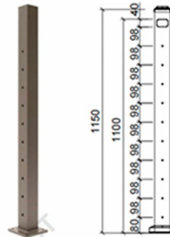
Aluminum Post With Drilled Holes For Cable Railing
